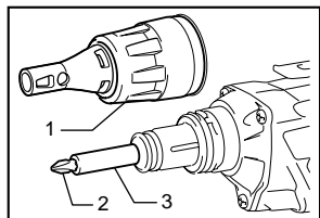
1. Locator 2. Bit 3. Magnetic bit holder
