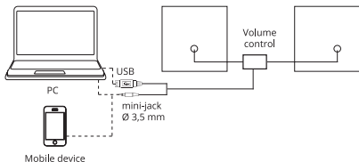
Fig. 1. Connection diagram
